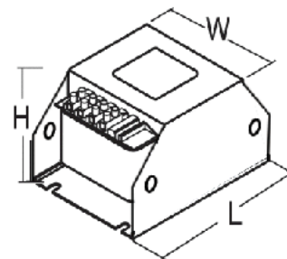
Ballast Diagram
